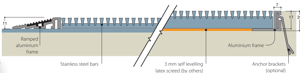
SURFACE MOUNTED
