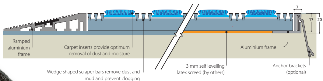
SURFACE MOUNTED
